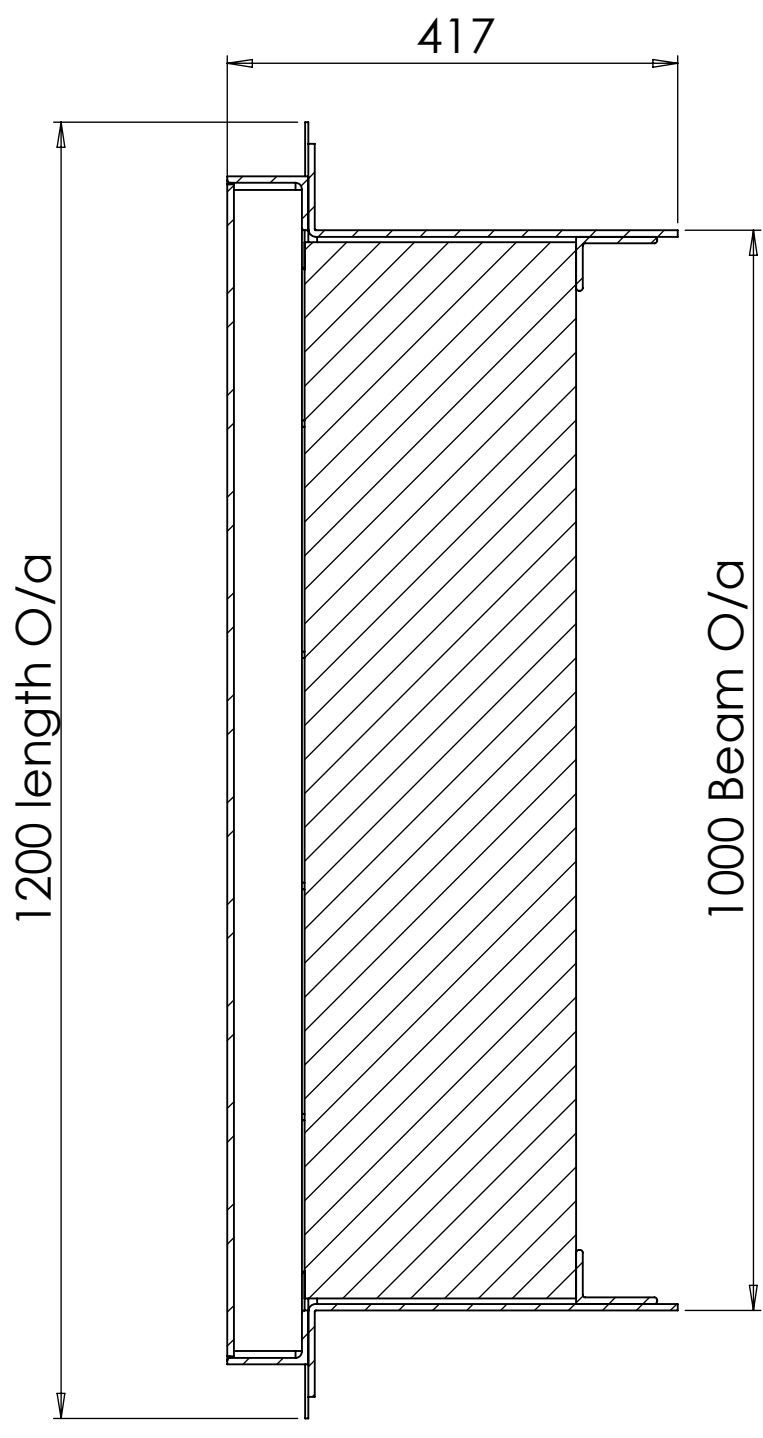
SECTION F-F SCALE 1 : 7
